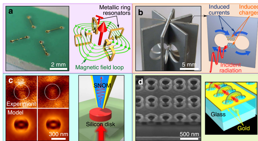
Fig. 3 Pioneering observations of dynamic toroidal and anapole excitations. (a) 2010. Observation of toroidal resonance. A photograph of the unit cell of microwave metamaterial exhibiting resonant toroidal dipole response, and a schematic of the unit cell supporting toroidal dipole excitation. Closed loops of magnetic field lines are characteristic of the toroidal response 1 . (b) 2013. Observation of anapole excitation. A photograph of the unit cell, with 8-fold rotational symmetry, of microwave metamaterial supporting anapole mode of excitation 30 . The schematic shows a fragment of the structure with a dumbbell cut. Electromagnetic waves polarized across the dumbbell gap induces electric (due to charges) and toroidal (due to currents) response in the structure. The emission of electric and toroidal excitations interferes destructively at the resonant frequency. (c) 2015. Observation of anapole mode in a silicon nano-disk 35 . The color maps show the electric field distribution in the disk, as mapped experimentally and modeled numerically, indicating the excitation of an anapole mode. The field was mapped using scanning near-field optical microscopy, as shown in the schematic. (d) 2018: Plasmonic metamaterial supporting anapole mode of excitation 41 . Scanning electron microscope image shows a cross-section of the nanostructure. It consists of a dumbbell-perforated section of the gold film with an additional gold split ring resonator below it. The schematic shows the unit cell of the metamaterial, as well as the sketch of the resonant mode, simultaneously supporting electric and toroidal dipoles
