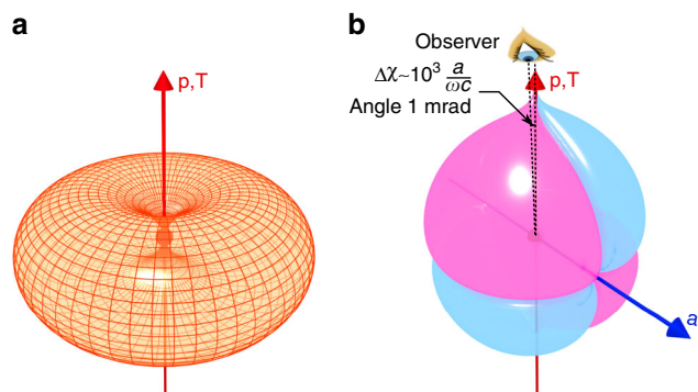
Fig. 4 Radiation of accelerated electric ( \mathbf{p} ) and toroidal ( \mathbf{T} ) dipoles. (a) The radiation patterns of non-accelerating electric ( \mathbf{p} ) and toroidal ( \mathbf{T} ) dipoles, oscillating at frequency \omega , are identical. However, emissions of accelerated oscillating electric and toroidal dipoles differ. Panel b shows the logarithmic plot of the difference between the ellipticity of emission of electric ( \chi_p ) and toroidal ( \chi_T ) dipoles accelerated with acceleration \mathbf{a} . Pink and blue colors corresponds to positive and negative ellipticity difference \Delta\chi = \chi_T - \chi_p ( c is the speed of light in the vacuum). Strongest effect due to ellipticity difference will be observable at small angle relative to dipole axis, where radiated power is still significant and ellipticity difference is large
