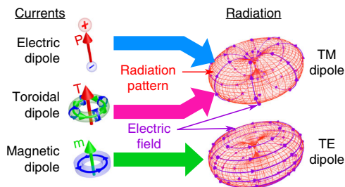
Fig. 2 Radiation patterns of the electric ( p ), magnetic ( m ) and toroidal ( T ) dipoles. Oscillating electric, magnetic, and toroidal dipoles have identical energy radiation patterns (emitted power per solid angle; red shells on the right). However, the electric and magnetic dipoles are distinguishable by the polarization state of the emitted light (TE - transverse electric; TM - transverse magnetic). Purple arrow lines on the surfaces of the shells show the direction of electric field oscillations. The electric and toroidal dipoles are indistinguishable by their far-field emission
