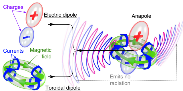
Fig. 1 Structure of a dynamic anapole. Anapole is a balanced superposition of electric and toroidal dipoles. Electric dipole corresponds to a pair of opposite charges. Toroidal dipole corresponds to a poloidal current on a torus. Anapole emerges when the fields radiated by the electric and toroidal dipoles cancel each other out
