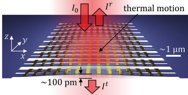
Figure 1. Thermal fluctuation of nanomechanical metamaterial optical properties. The photonic metamaterial is an array of beams of nanoscale width and thickness in the xy plane. The beams, typically a few tens of microns long, support a periodic array of optical resonators of nanoscale (subwavelength) dimensions. The optical properties of such arrays can be controlled via nanostructural reconfiguration driven by external stimuli such as electromagnetic forces, optical and acoustic waves. [2–4,7,8] Piezometric thermal displacements of the individual beams also modulate the optical properties of the metamaterial, causing small fluctuations of its transmittance and reflectance.
