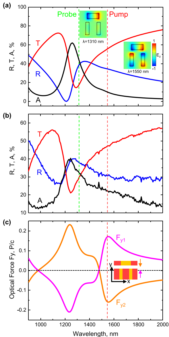
FIG. 2. Optical properties of the reconfigurable metamaterial. (a) Simulated and (b) measured reflection (R), transmission (T), and absorption (A) spectra of the nanostructure. (c) In-plane optical forces per unit cell in units of P/c according to Maxwell stress tensor calculations, where P is the incident power and c is the speed of light in vacuum. Pump and probe wavelengths are indicated by dashed lines, and the insets of panel (a) show the optically induced charge distributions at these wavelengths in terms of the normalized electric field perpendicular to the unit cell's surface.
