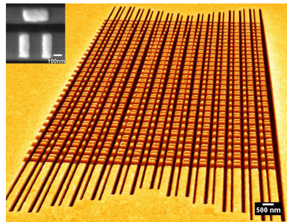
FIG. 1. Optically addressable nanomechanical metamaterial. Scanning electron micrograph of the nanostructure and its unit cell (inset). Yellow represents gold and brown represents silicon nitride.
