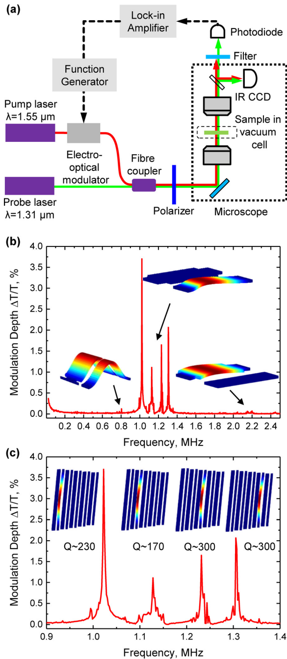
FIG. 3. Selective actuation of metamaterial strings with light. (a) Schematic of the experimental setup for actuating individual nanostrings with a 1550 nm wavelength pump laser modulated at frequency f and detecting the resulting modulation of a transmitted 1310 nm CW probe laser with a lock-in amplifier locked to the same frequency. (b) and (c) Detected transmission modulation \Delta T/T at the probe wavelength as a function of the pump modulation frequency f . Insets show COMSOL simulations of the mechanical eigenmodes corresponding to the observed resonances.
