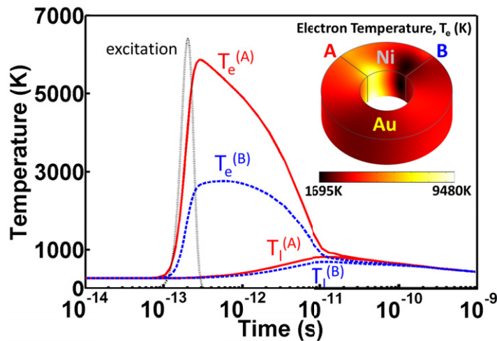
Figure 2. Temporal temperature profiles upon irradiation by a light pulse. Electron ( T_e ) and lattice ( T_l ) temperatures at the hot (solid red, A) and cold (dashed blue, B) junctions of the ring. The pulse fluence is 11.3 \text{ J m}^{-2} and evolves as shown by the dotted curve. A snapshot of the electron temperature on the ring surface is shown in the inset at the time corresponding to the maximum of T_e in the hot junction A.
